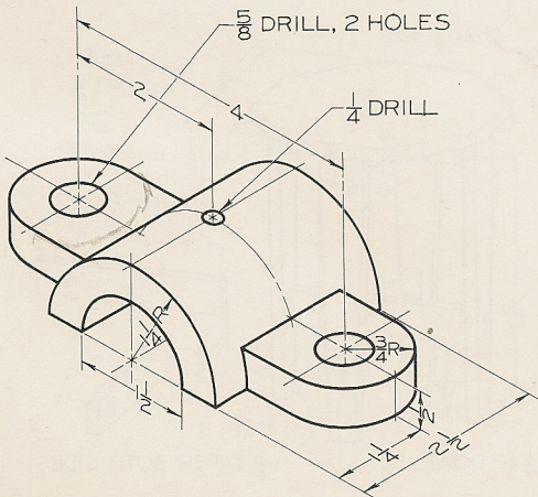
Fig. 7-67. Bearing Cap.*
