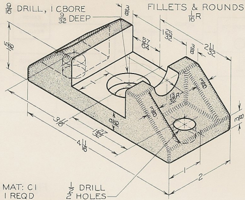
Fig. 10-31. Clamp Block.*
