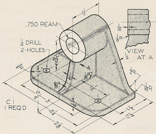
Fig. 10-30. Shaft Bracket.*
